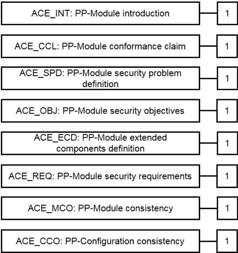
Figure 9 - ACE: Protection Profile Configuration evaluation class decomposition
